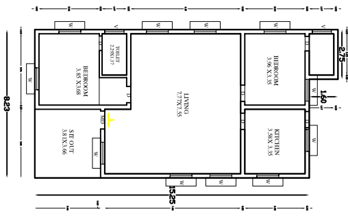
PROPOSED GROUND FLOOR
