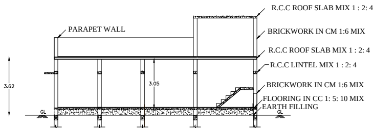
SECTION ON AB &( HALF ELEVATION)
