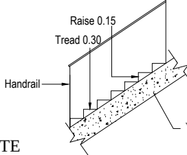
STAIRCASE DETAILS
