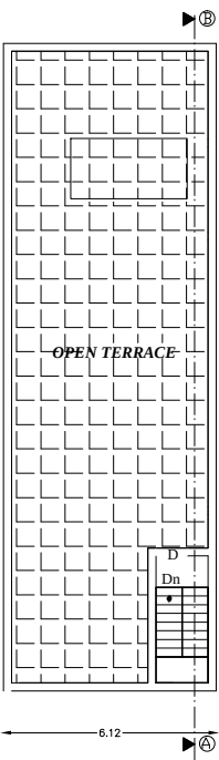
TERRACE FLOOR PLAN
