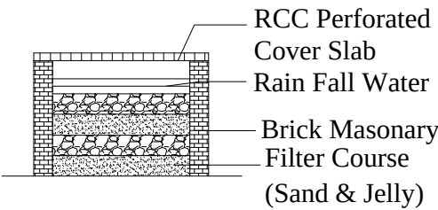
PLAN SECTION OF RECHARGE TRENCH METHOD
