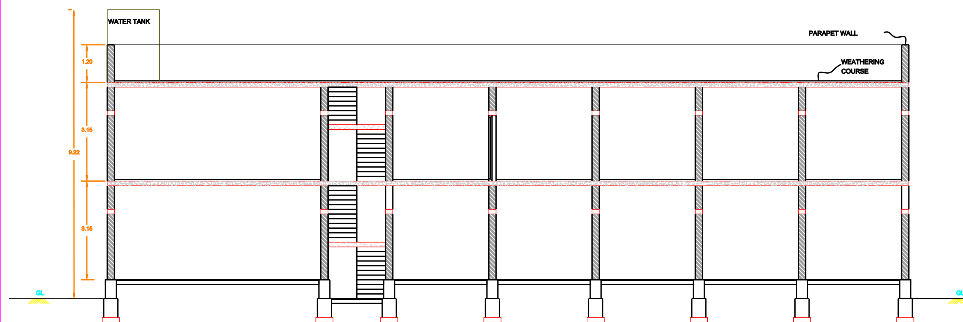
SECTION- BB
