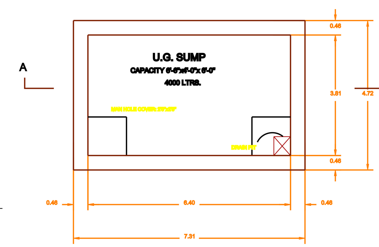
SUMP DETAIL
