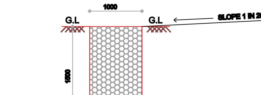
SECTION OF PEBBLE TRENCH
