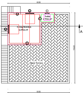
PRO.SECOND FLOOR PLAN
