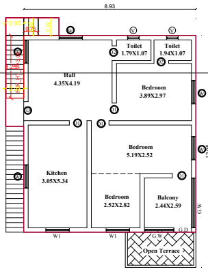
EXG.FIRST FLOOR PLAN
