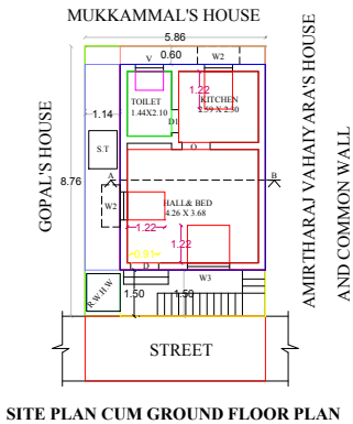
SITE PLAN CUM GROUND FLOOR PLAN
