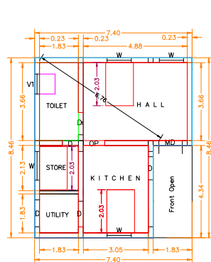
PRO.GROUND FLOOR PLAN SCALE 1:100
