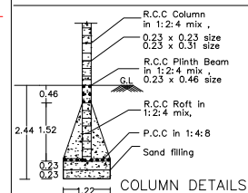
COLUMN DETAILS
