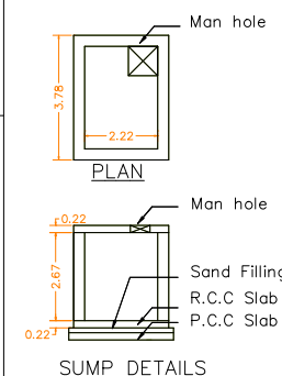
SUMP DETAILS
