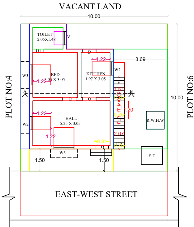
SITE PLAN CUM GROUND FLOOR PLAN
