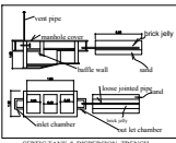
SEPTIC TANK & DISPOSAL TRENCH
