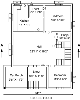
GROUND FLOOR
