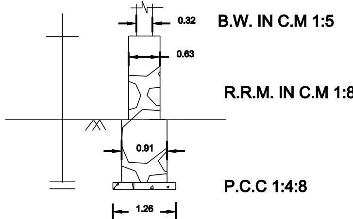
COLUMN DETAILS
