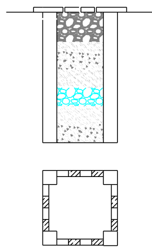
PLAN & SECTION OF RAIN WATER COLLECTION WELL
