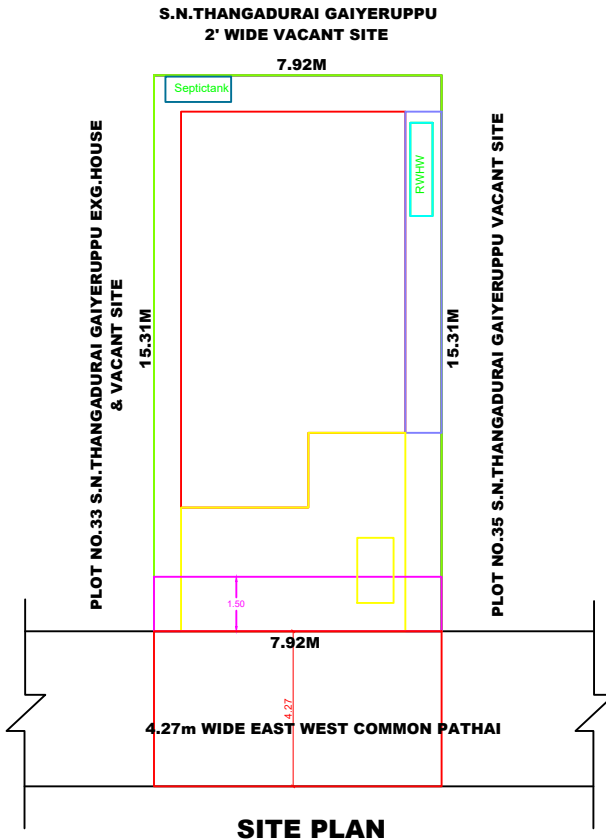
SITE PLAN
