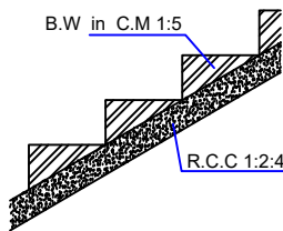
STAIRCASE
