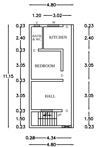
PRO GROUND FLOOR PLAN
