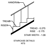
STAIRCASE DETAILS NTS
