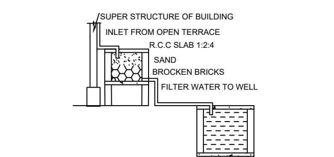
RAINWATER HARVESTING
