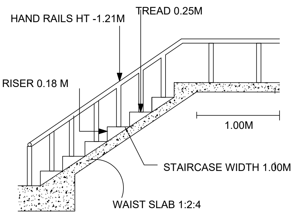
STAIRCASE DETAILS
