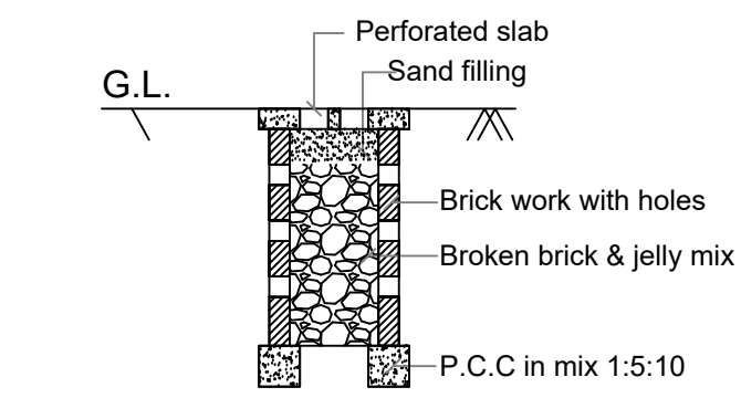
RAINWATER HARVESTING
