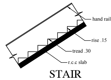
STAIR
