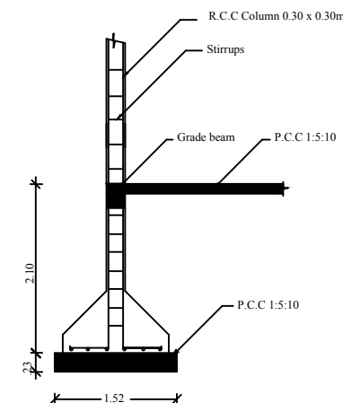
Column Detail
