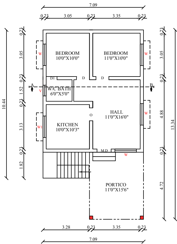
PROPOSED G.F. PLAN
