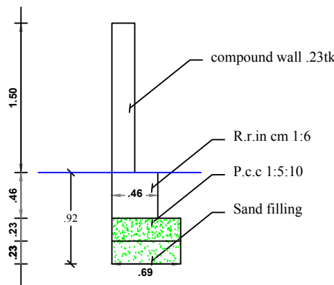
Compound Wall Detail
