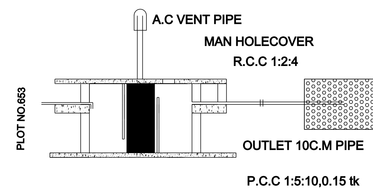
SECTION
