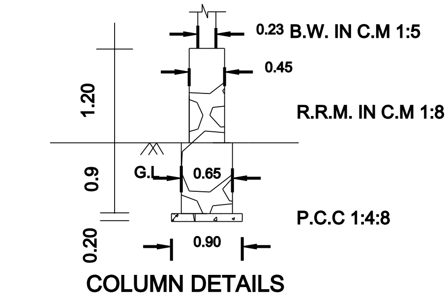
COLUMN DETAILS
