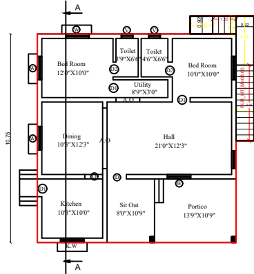
EXG.GROUND FLOOR PLAN
