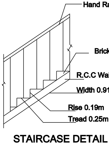
STAIRCASE DETAIL
