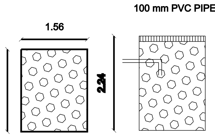
PLAN & SECTION OF RAINWATER COLLECTION TANK
