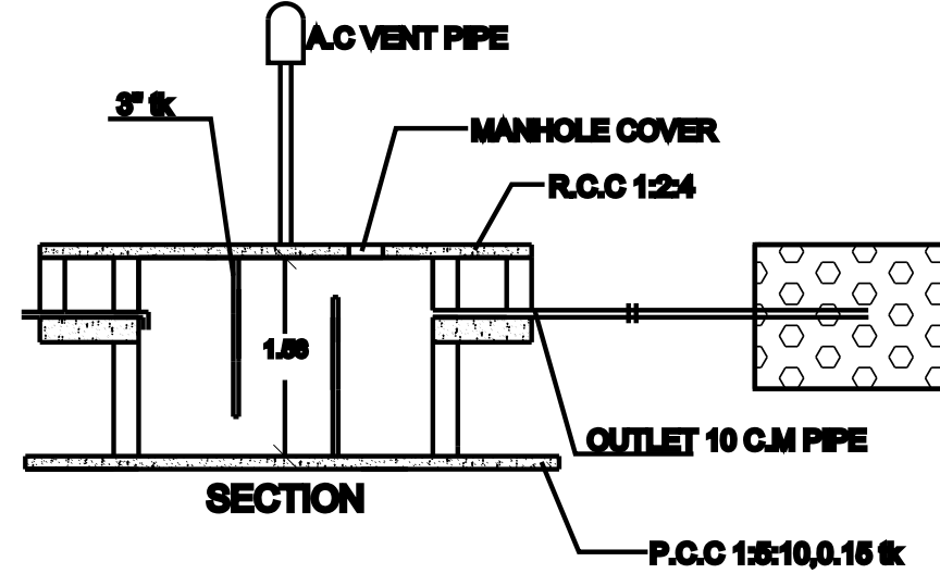
SECTION
