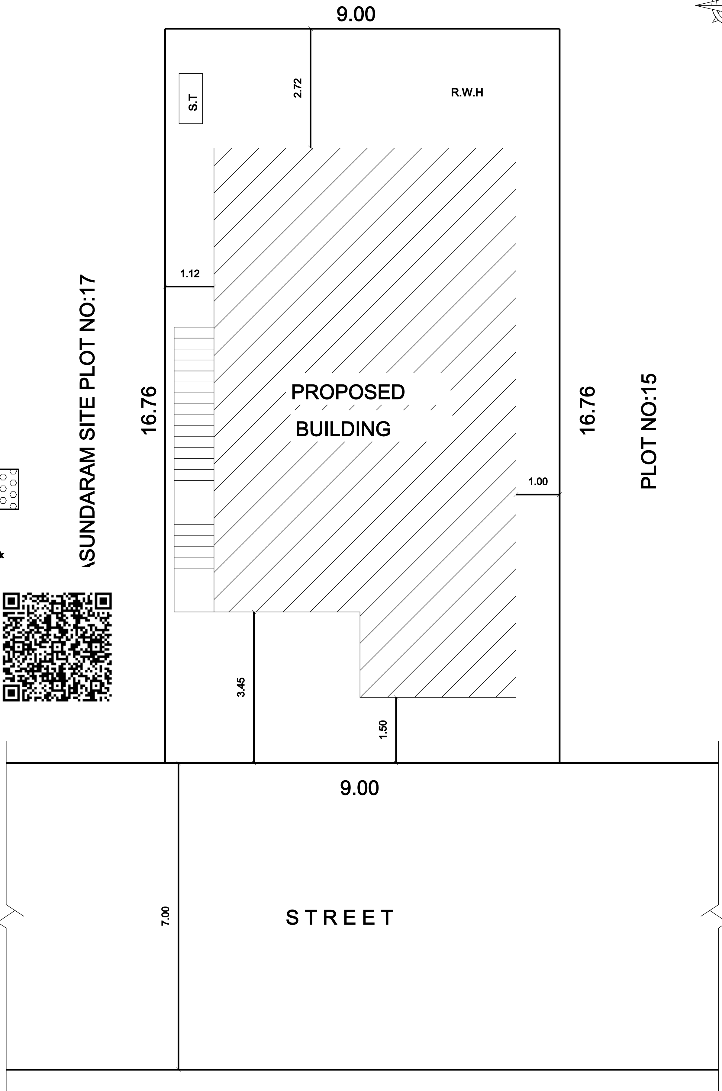
SITE PLAN
