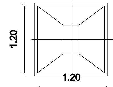
PLAN R.C.C. FOOTING DETAILS
