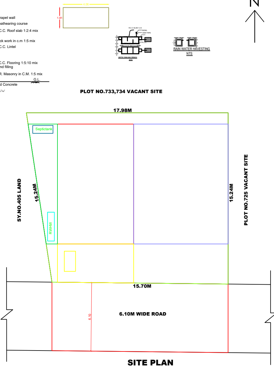
SITE PLAN
