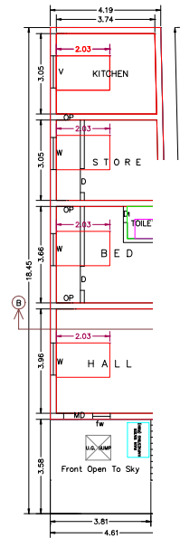
PRO.G.FLOOR PL SCALE 1:100
