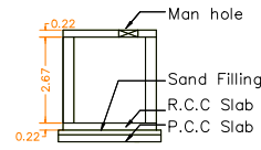
SUMP DETAILS
