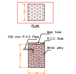
SECTION OF RAINWATER COLLECTION TANK
