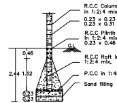
COLUMN DETAILS
