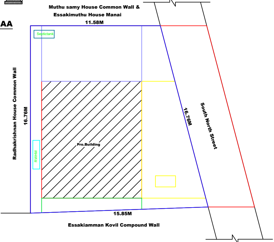
SITE PLAN
