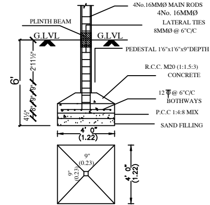
FOUNDATION DETAIL (SCALE: 1:50)
