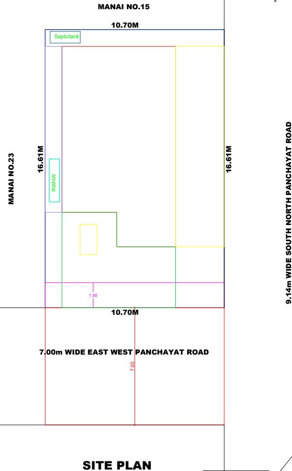
SITE PLAN
