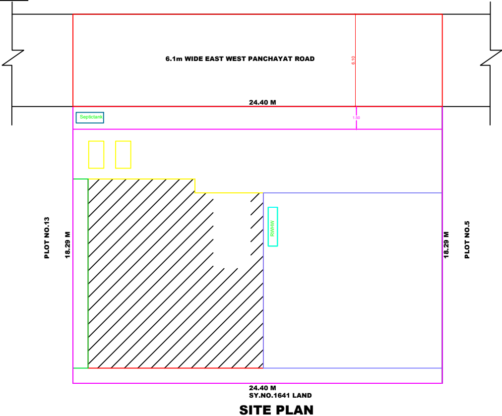
SITE PLAN
