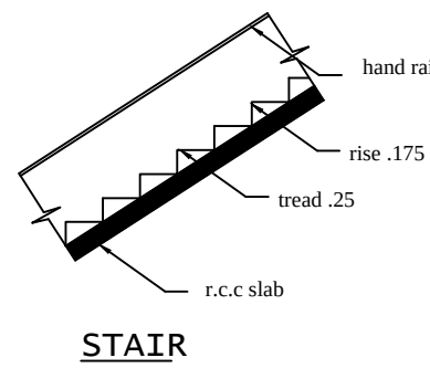
STAIR
