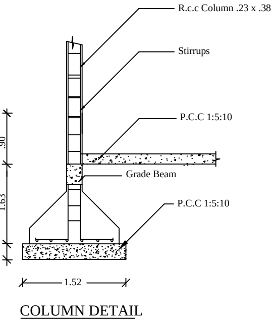
COLUMN DETAIL
