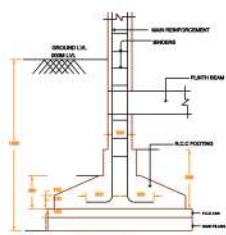
TYPICAL SECTION OF
