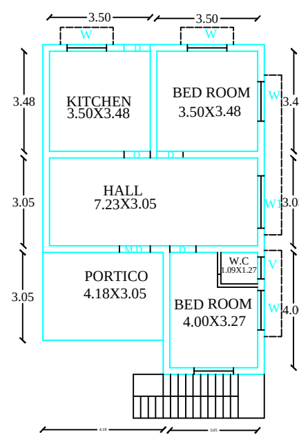
PROPOSED GROUND FLOOR
