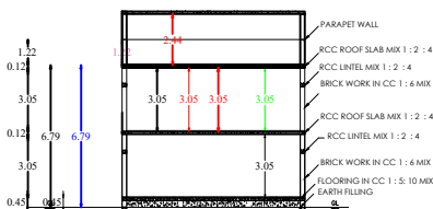
SECTION ON AB & ( HALF ELEVATION)
