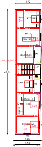
PRO FIRST FLOOR PLAN
