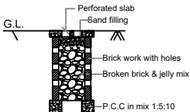
RAINWATER HARVESTING
