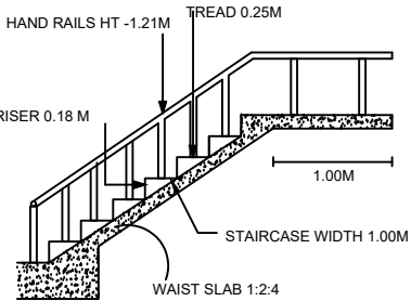
STAIRCASE DETAILS
