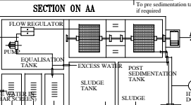
SECTION ON AA SEWAGE TREATMENT PLANT DETAILS WASTE WATER RECYCLING UNIT
