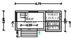
PRO. GROUND FLOOR PLAN
