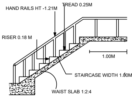
STAIRCASE DETAILS
