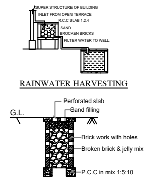
RAINWATER HARVESTING
