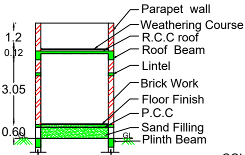
SECTION AB
