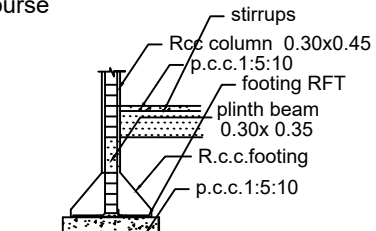
COLUMN DETAILS
