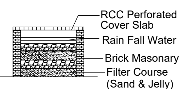
SECTION OF RECHARGE TRENCH METHOD
