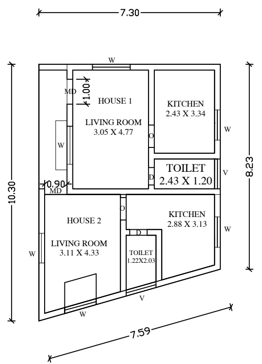
PROPOSED RESIDENTIAL FIRST FLOOR PLAN
