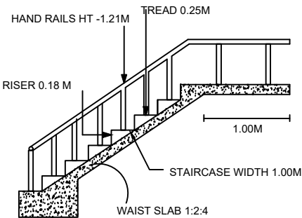
STAIRCASE DETAILS
