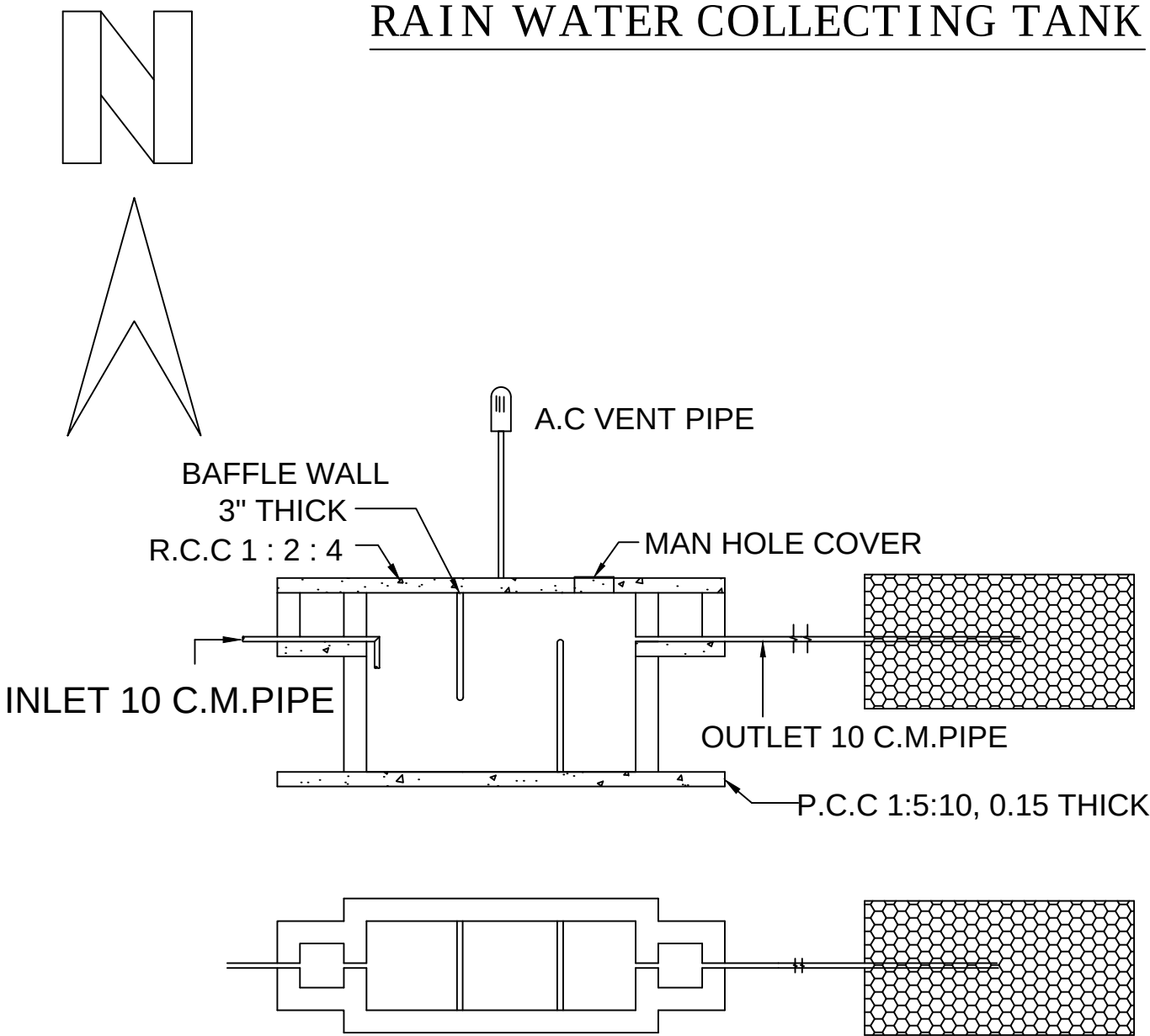
SEPTIC TANK & TRENCH
