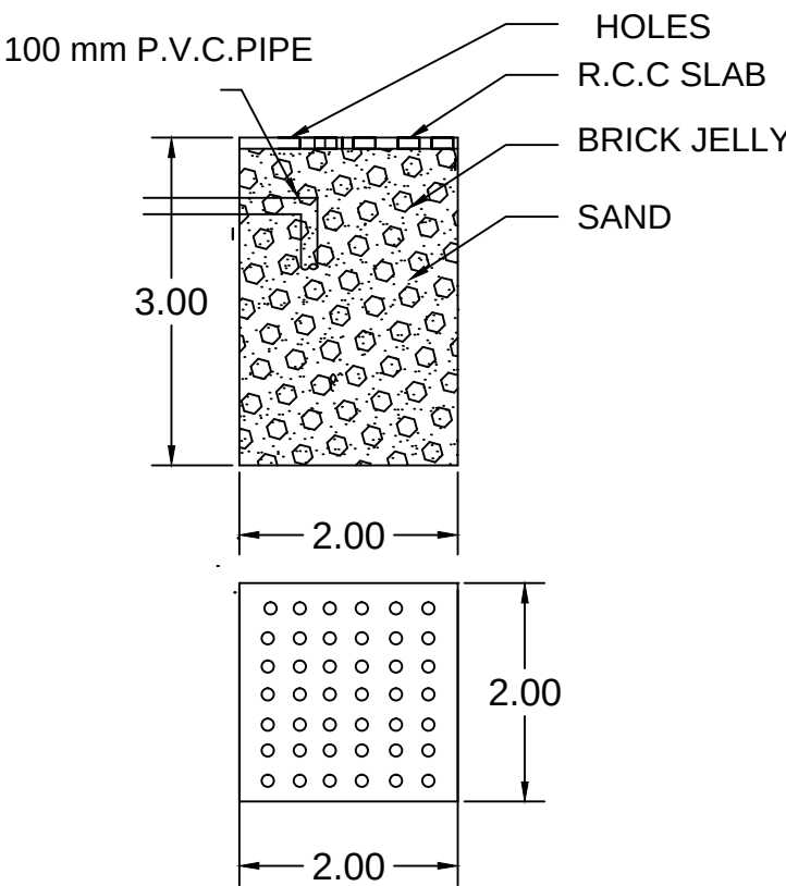
RAIN WATER COLLECTING TANK
