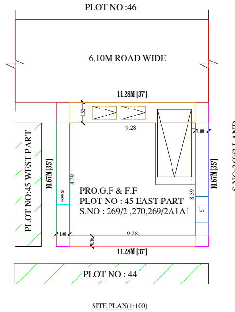
SITE PLAN (1:100)
