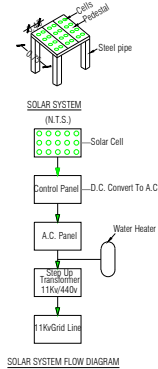
SOLAR SYSTEM FLOW DIAGRAM
