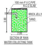
SECTION OF RAIN WATER COLLECTING TANK
