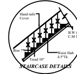
STAIRCASE DETAILS
