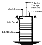
SECTION ON SOAKPIT
