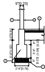
FOUNDATION DETAILS
