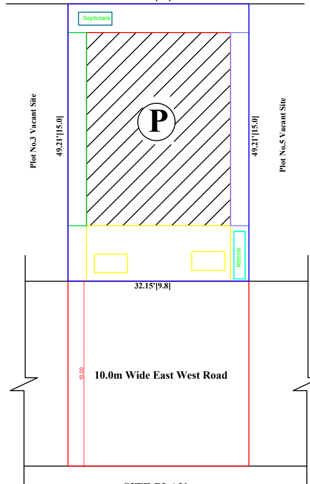
SITE PLAN
