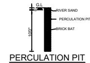
PERCOLATION PIT
