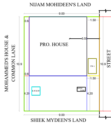
SITE PLAN
