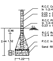
COLUMN DETAILS
