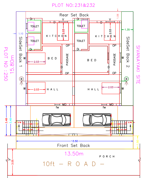
SITE CUM GROUND FLOOR PLAN SCALE 1:100
