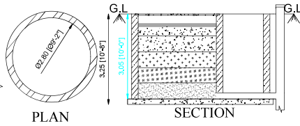
RAIN WATER HARVESTING OF RECHARGE TRENCH METHOD
