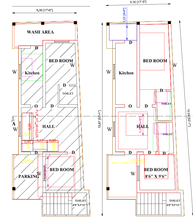
PRO.& EX.GROUND FLOOR PLAN FIRST FLOOR PLAN
