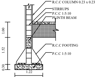
COLUMN DETAILS
