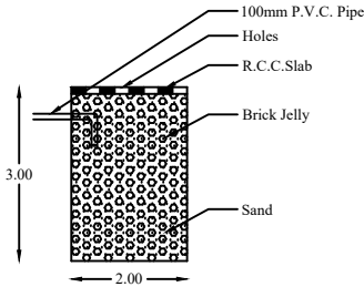
SECTION OF RAIN WATER COLLECTING TANK
