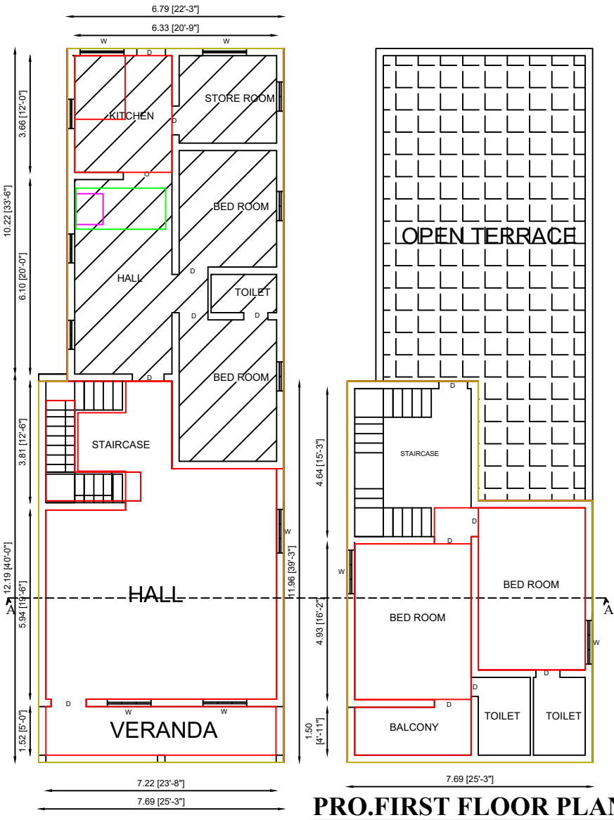
EX. AND PROPOSED GROUND FLOOR PLAN
