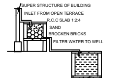
RAINWATER HARVESTING
