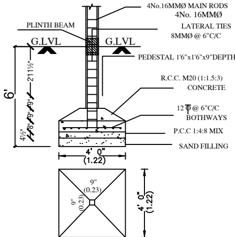
FOUNDATION DETAIL
