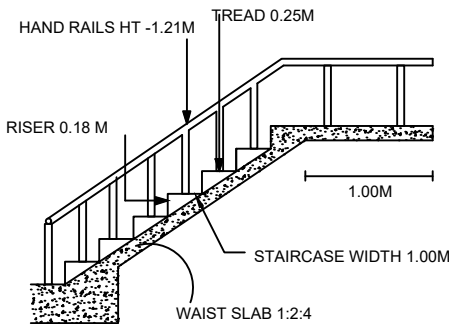
STAIRCASE DETAILS
