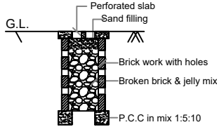
RAINWATER HARVESTING
