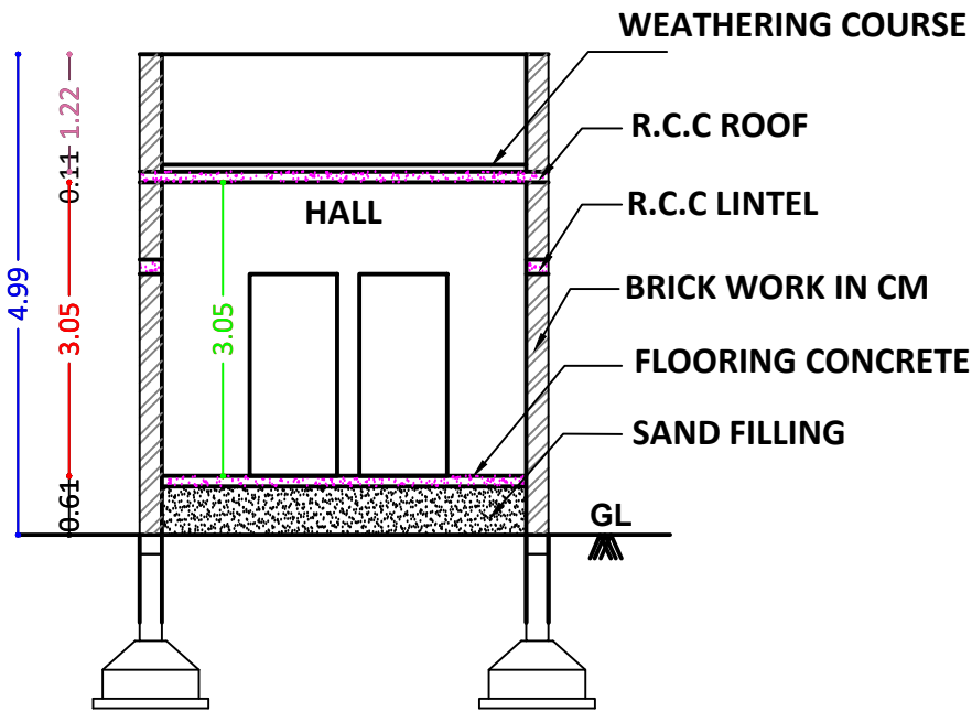
SECTION AB
