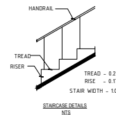
STAIRCASE DETAILS NTS
