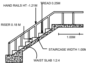
STAIRCASE DETAILS
