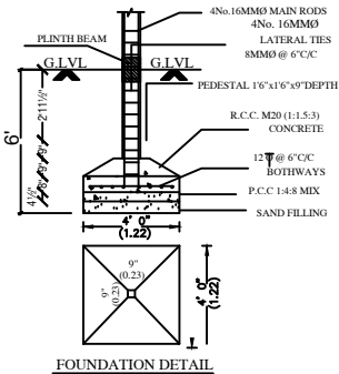
FOUNDATION DETAIL
