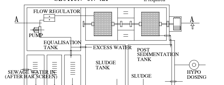
PLAN SEWAGE TREATMENT PLANT DETAILS WASTE WATER RECYCLING UNIT
