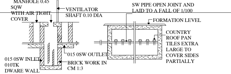
DETAILED DRAWING FOR SEPTIC TANK WITH DISPERSION TRENCH 225 GALLONS CAPACITY OF 1000 LITRES
