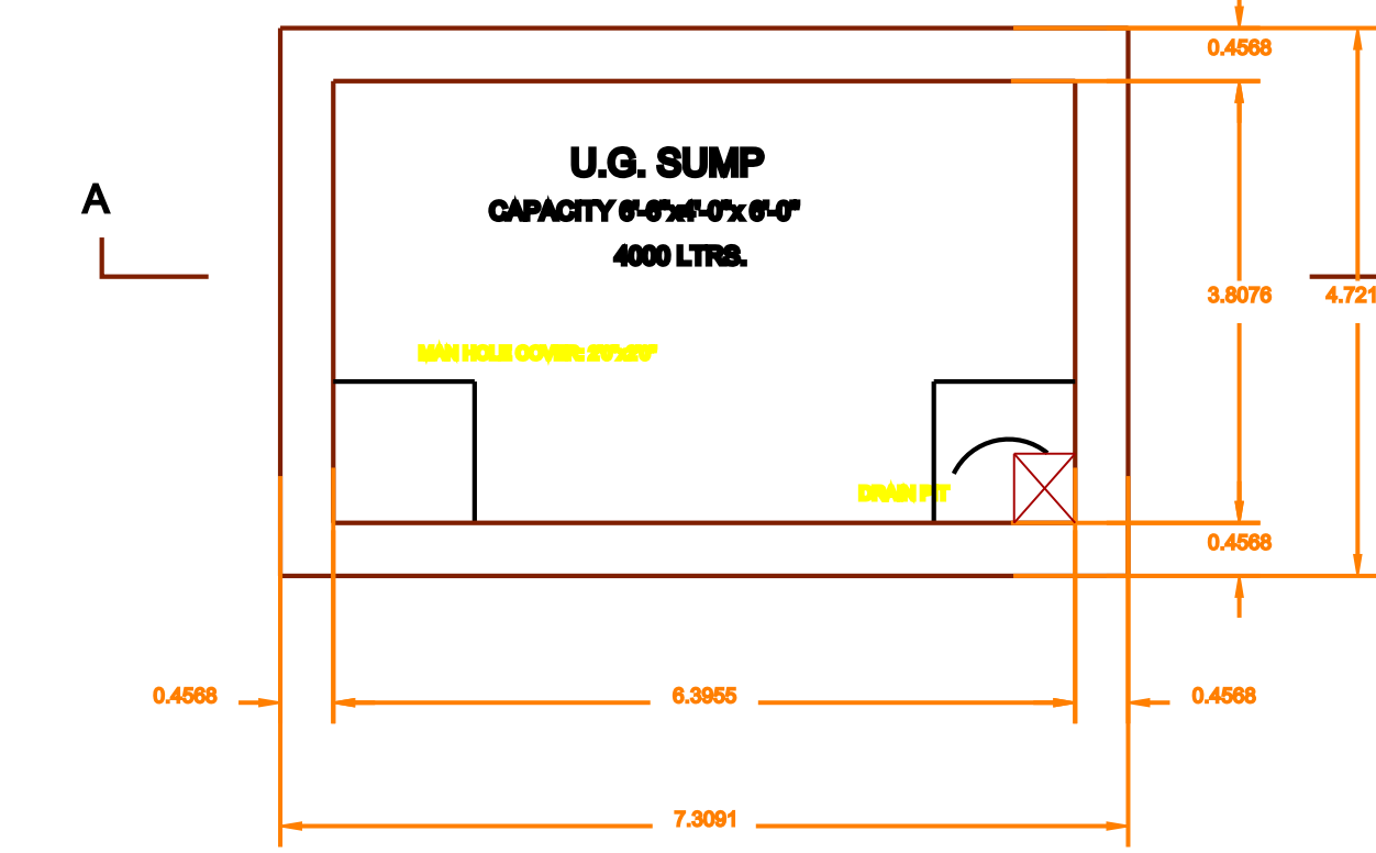
SUMP DETAIL
